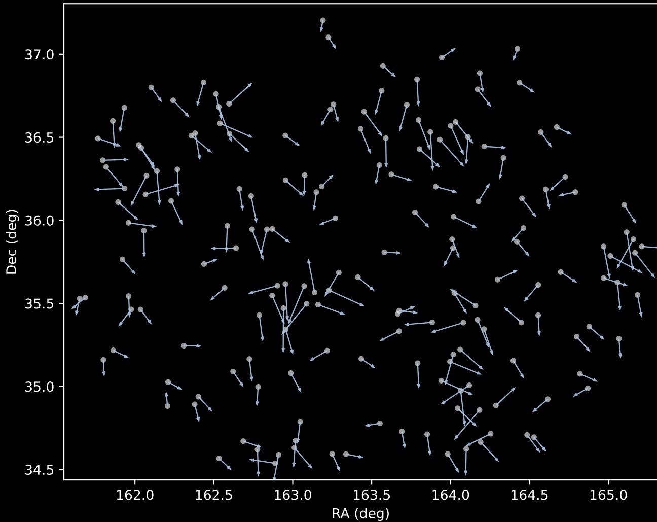
APOGEE DR17 Cluster 1 Proper Motion Vectors (n=175)
