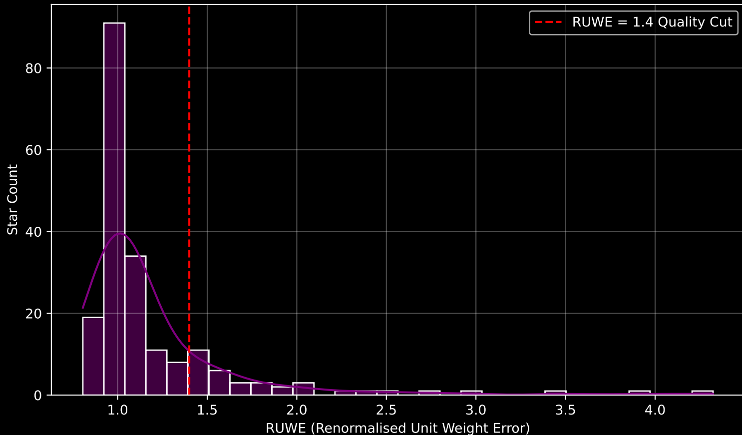
GAPOGEE DR17 Field [CA_162-11_btx] RUWE Distribution (n= 199)
