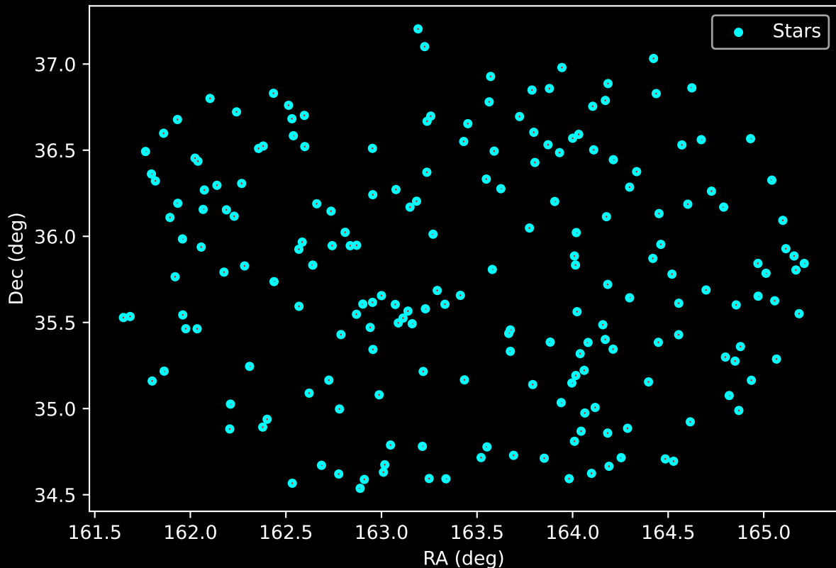
APOGEE DR17 Field: [CA_162-11_btx] Proper Motion Vectors for Gaia Star Field (n= 199)
