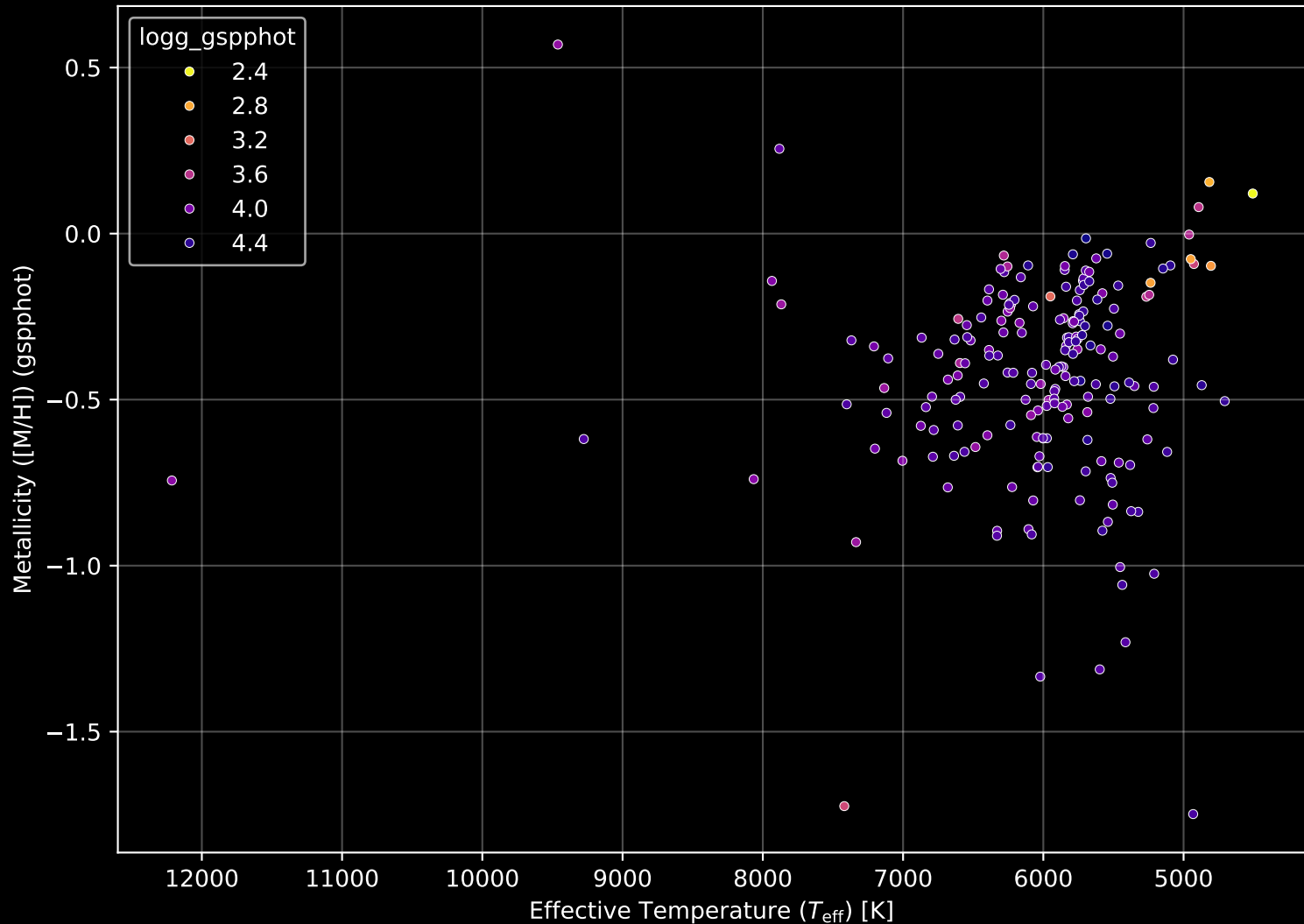
APOGEE DR17 Field: [CA_162-11_btx] Stellar Population Parameters (n= 199)
