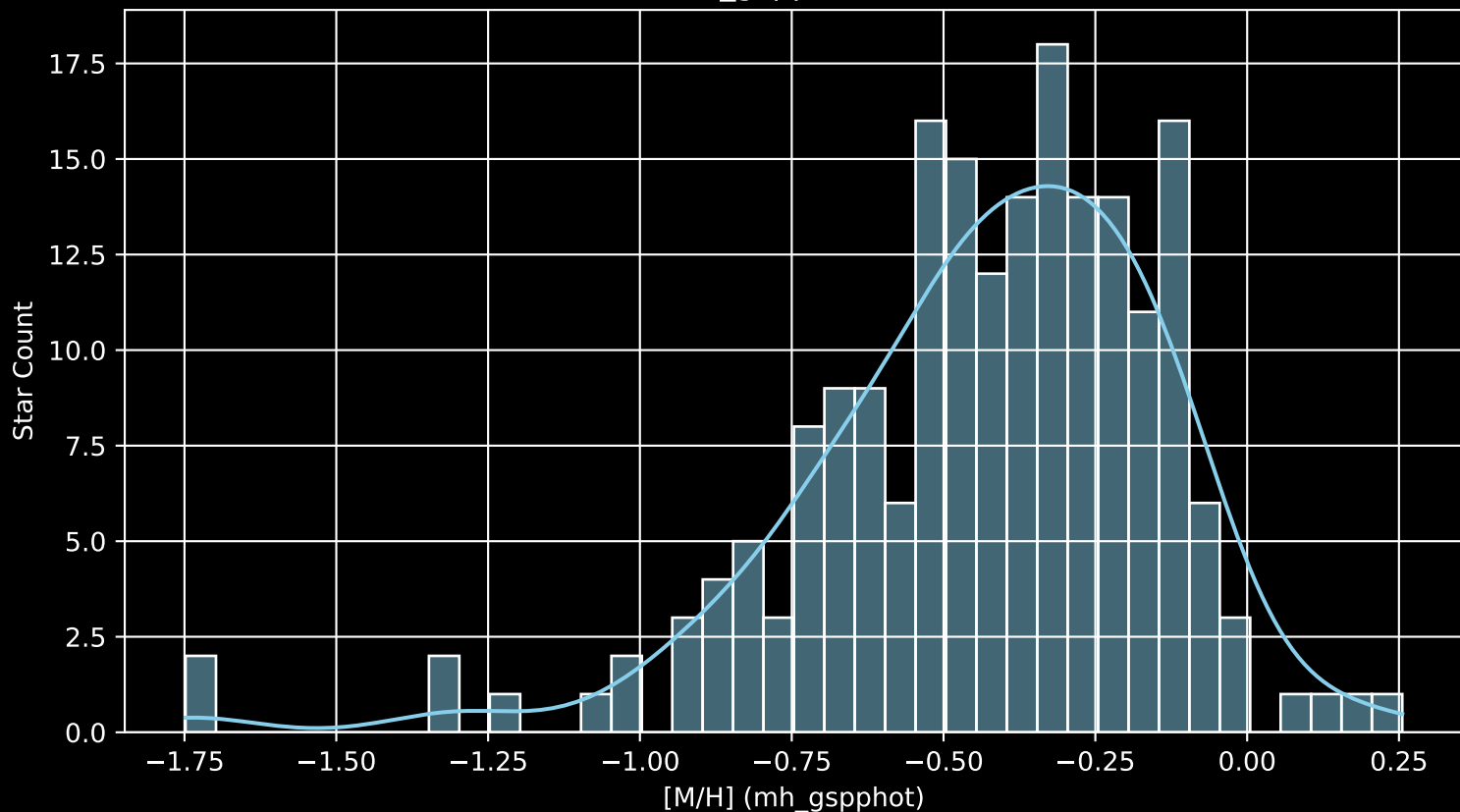
APOGEE DR17 Field: [CA_162-11_btx [M/H] (mh_gspphot) (n= 198)
