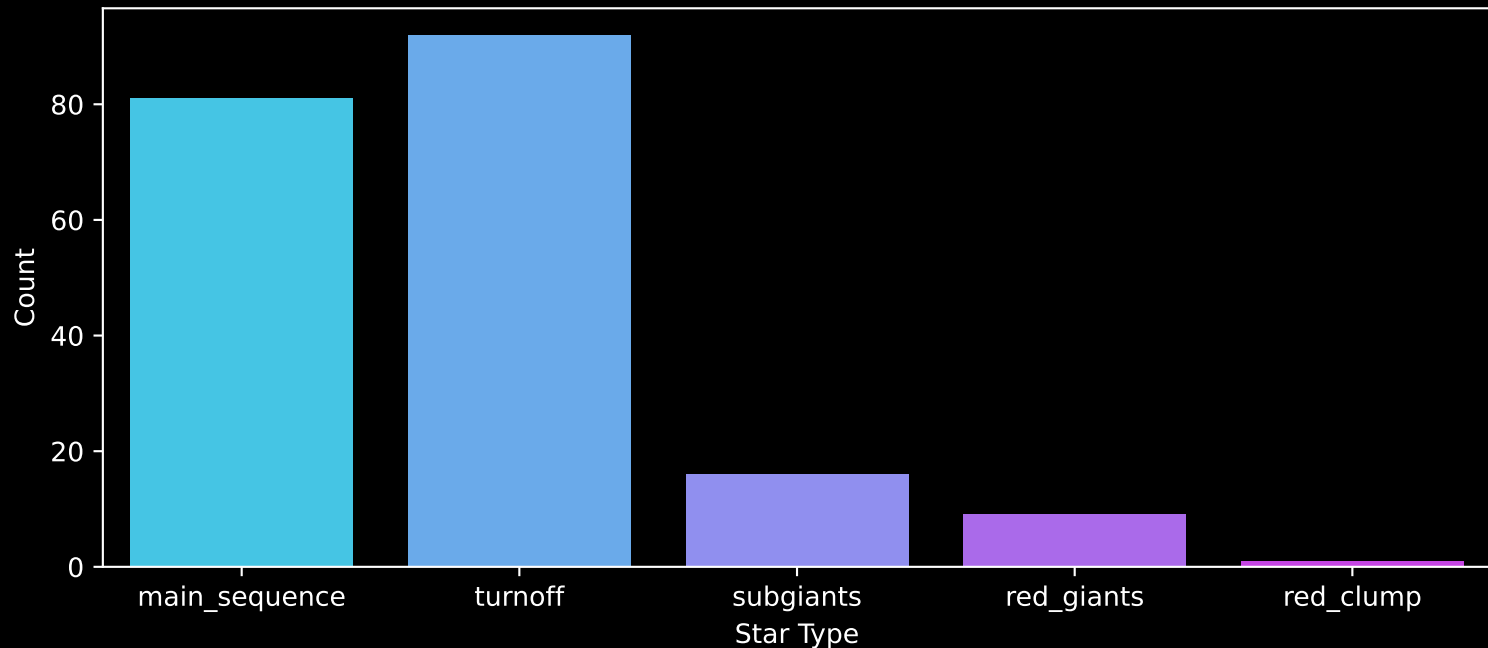
APOGEE DR17 Field: [CA_162-11_btx] Count plot of Star Type
