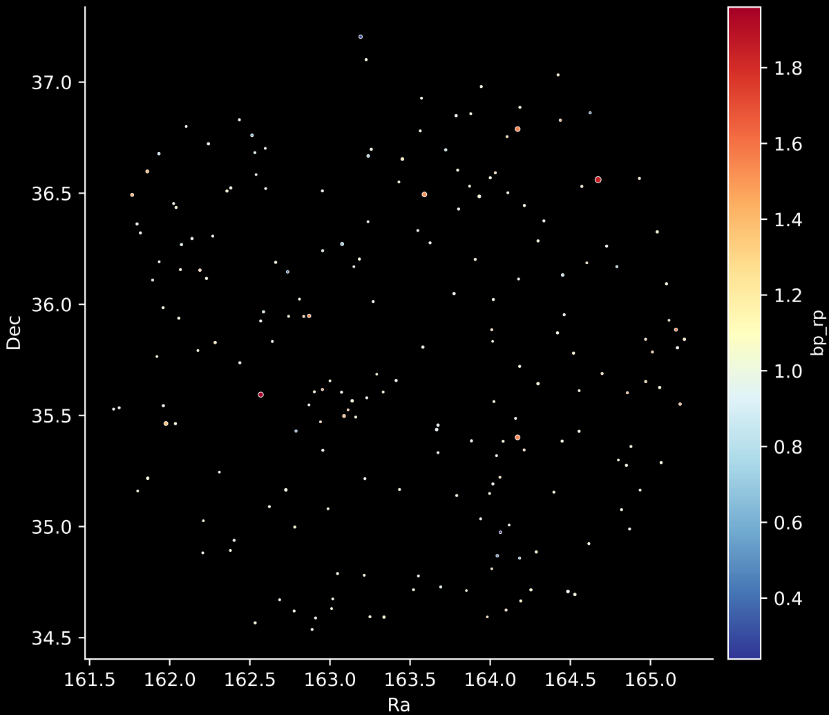
APOGEE DR17 Field: [CA_162-11_btx] Stars: 199
