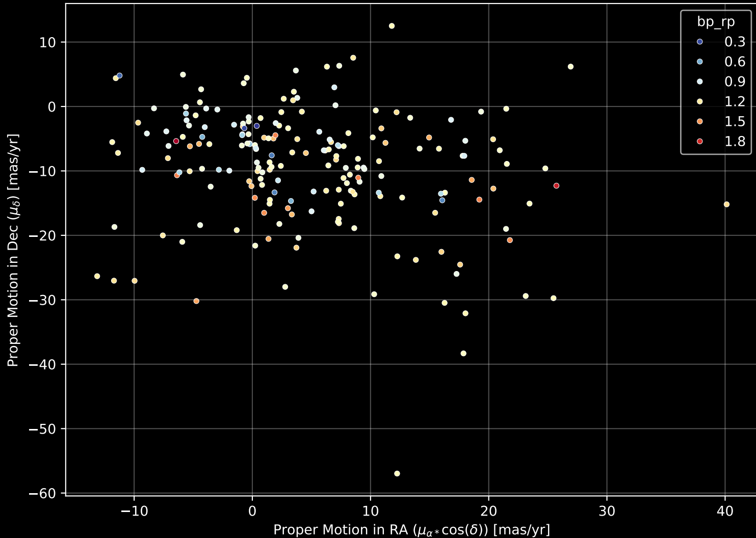
APOGEE DR17 Field: [CA_162-11_btx] Proper Motion Diagram (n= 199)
