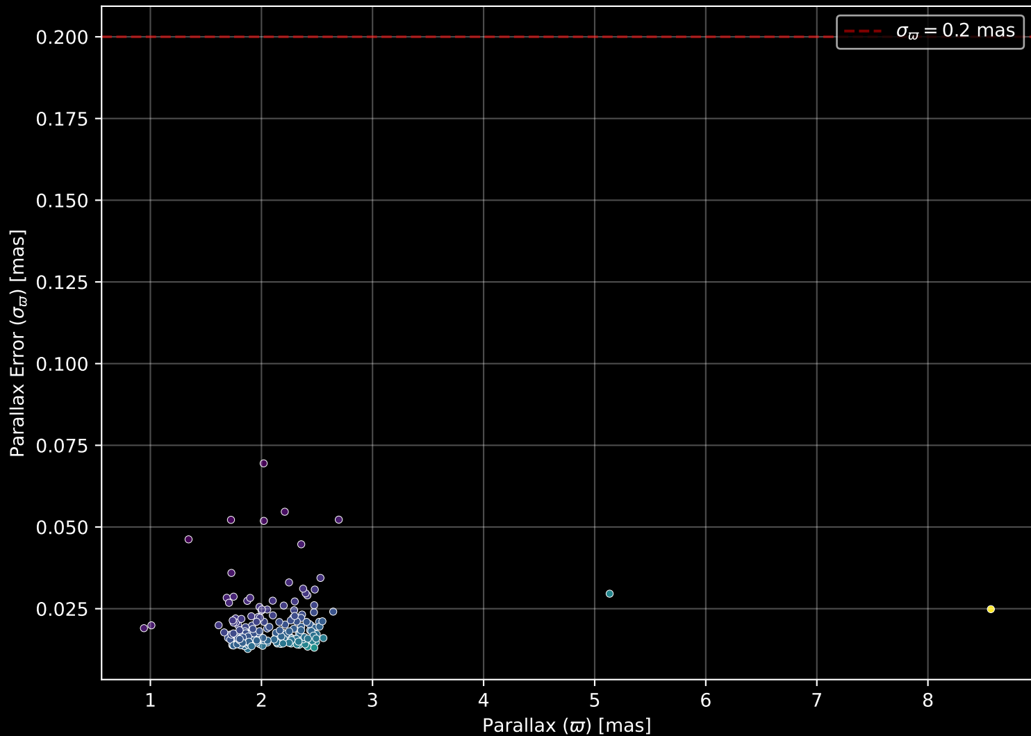
APOGEE DR17 Field: [CA_162-11_btx] Parallax Quality (n= 199)
